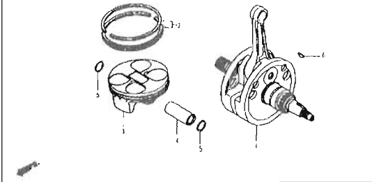
BLOCK No. E-15 CRANKSHAFT/PISTON
