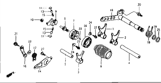
BLOCK No. E-18 GEARSHIFT DRUM
