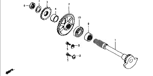
BLOCK No. E-16 BALANCER
