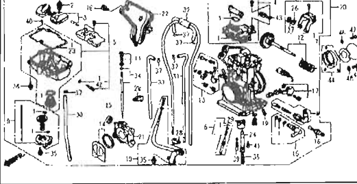
BLOCK No. E-20 CARBURETOR
