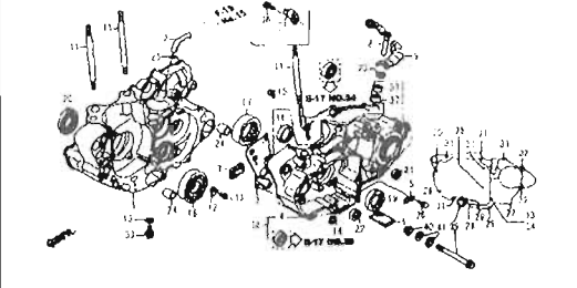
BLOCK No. E-14 CRANKCASE
