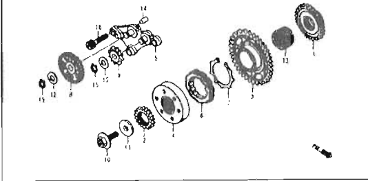
BLOCK No. E-13 STARTING CLUTCH
