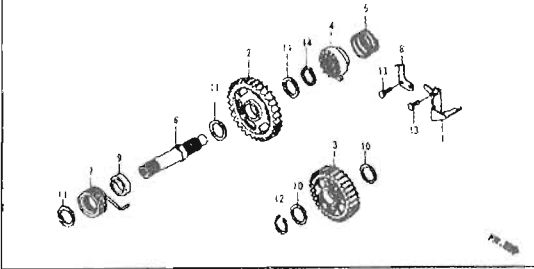
BLOCK No. E-19 KICK STARTER SPINDLE
